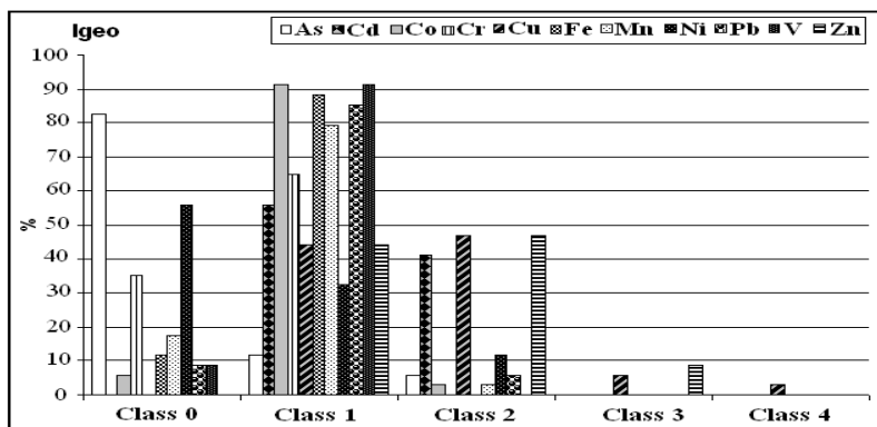
Figure 3. I_{geo} values for studied elements.
