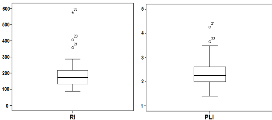
Figure 4. RI and PLI in river sediments.
