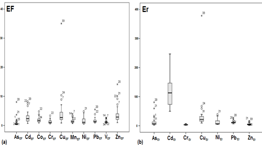
Figure 2. Values of EF (a) and Er (b) for studied elements.
