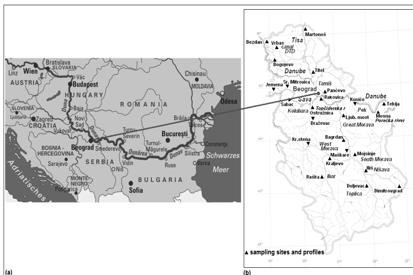
Figure 1. Danube watershed and sampling locations.
