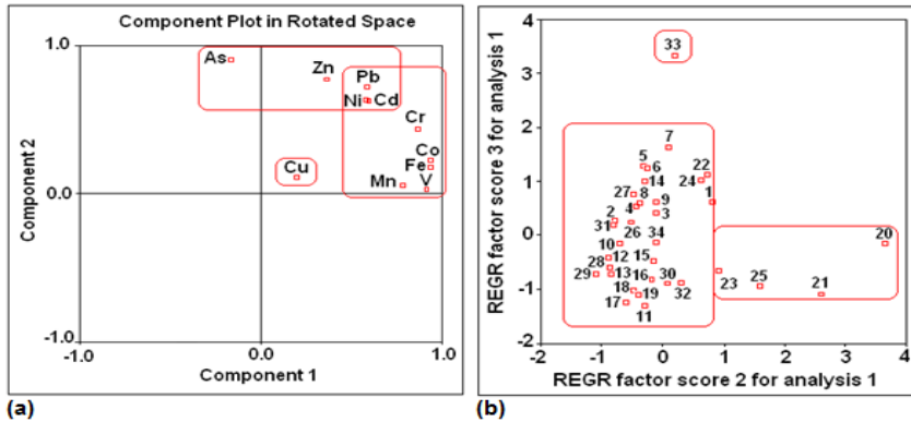
Figure 5. Results of PCA analysis.
